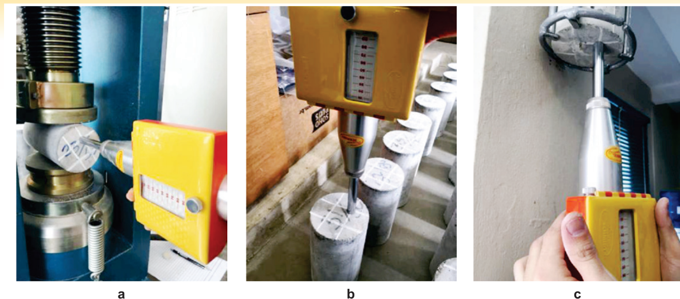
Figure 4 Sclerometry test performed in three positions: (a) Position 1(→) (b) vertical downwards (Position 2) and (c) vertical upwards (Position 3)
