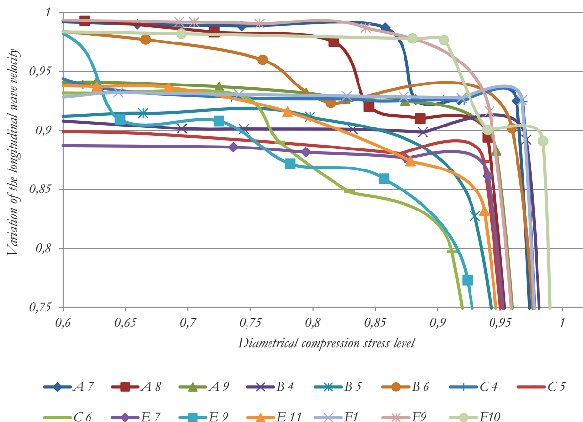
Figure 6 Summary of longitudinal wave behavior in concrete samples subjected to split test
