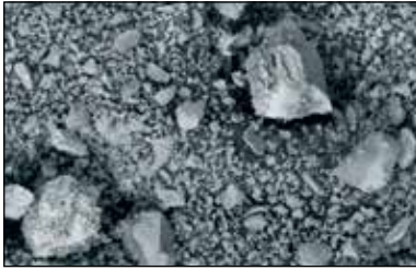
Cover: SEM IMAGE OF HEAT TREATED ORNAMENTAL STONE PROCESSING WASTE
