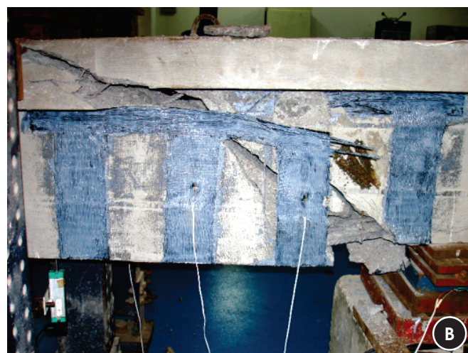
Figure 11 – Beam failure: a) VR2; b) VII-1
